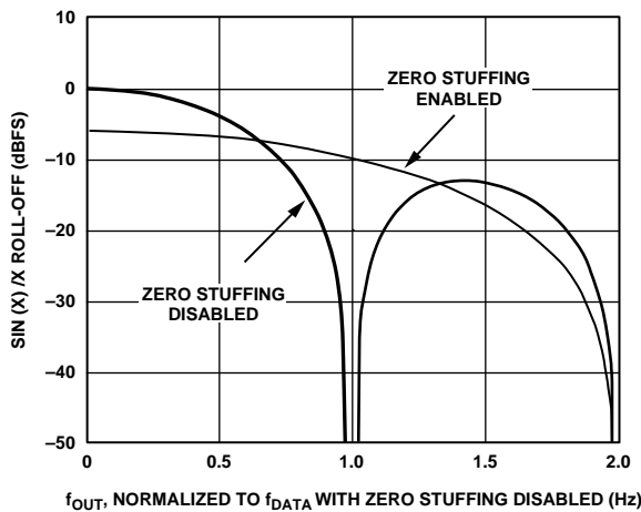
Figure 75. Effect of Zero Stuffing on DAC's SIN(x)/x Response
